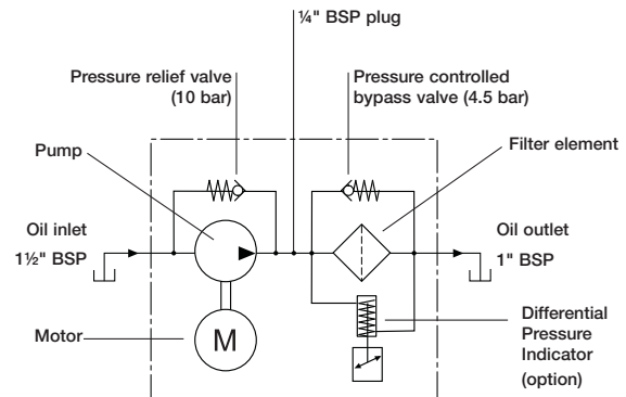
Pall Ultiplead® Filtration Unit
